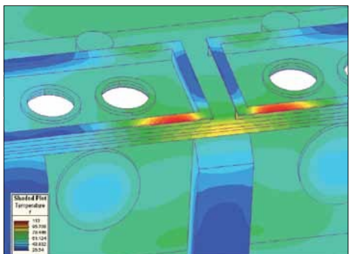
Thermovision of the LV turrets of an ABB 500 MVA single-phase GSU transformer (left), and the corresponding temperature distribution calculated by ABB (right).
